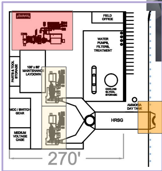
Synapse Data Center - (1) 140MW NG Plant Layout Example
